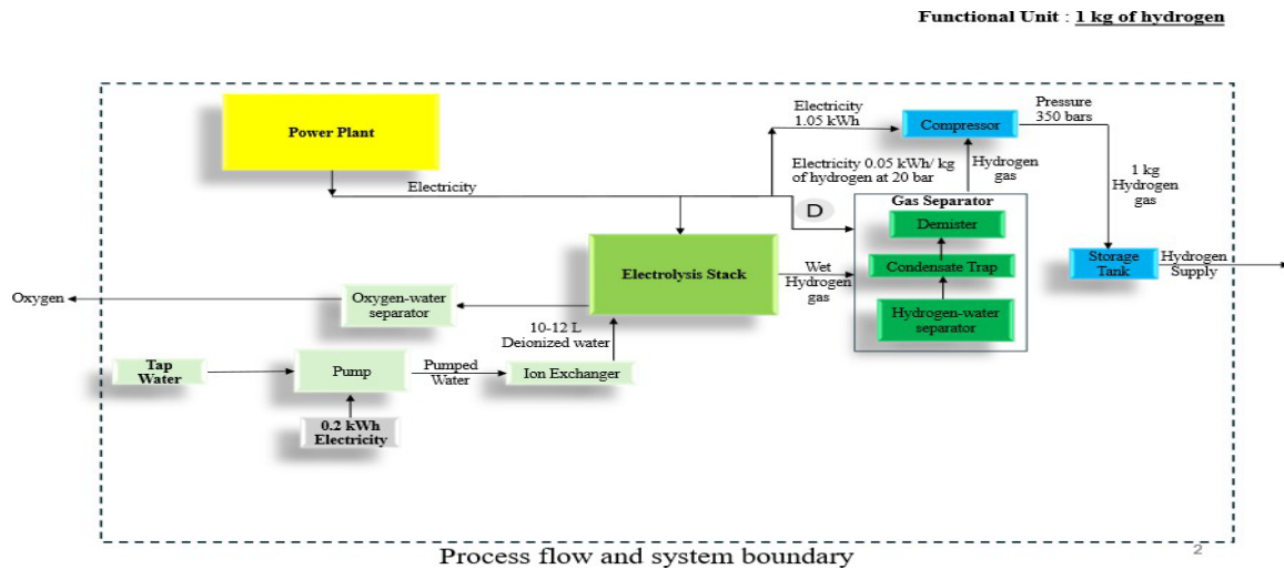
Figure 1 Process flow and system boundary
