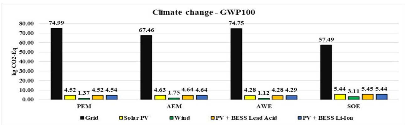
Figure 2 Global Warming Potential (GWP)
