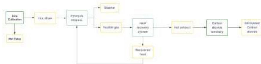
Figure 3. System boundary of Scenario 3 Biochar production
