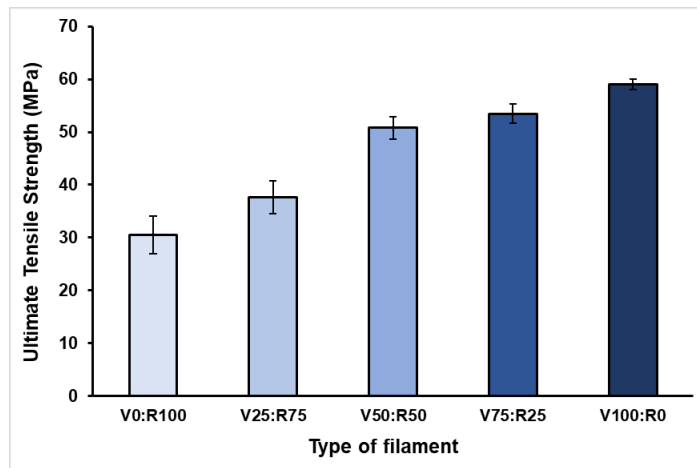
Figure 2. Ultimate tensile strength of the tested specimens
