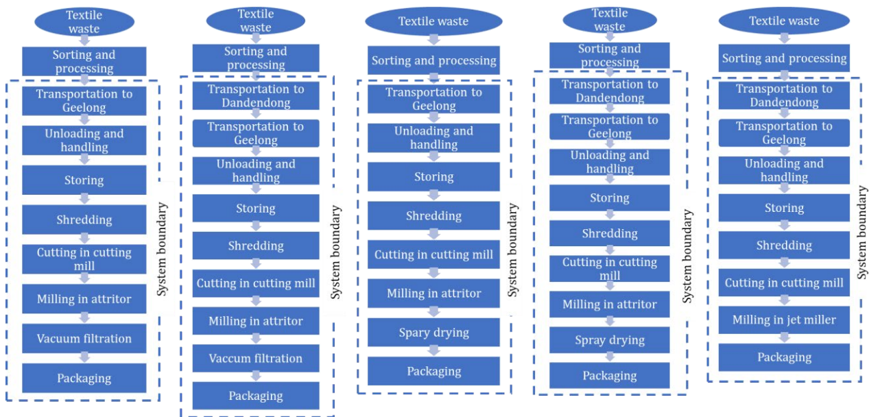
Figure 1- Process mapping for process P1-A
