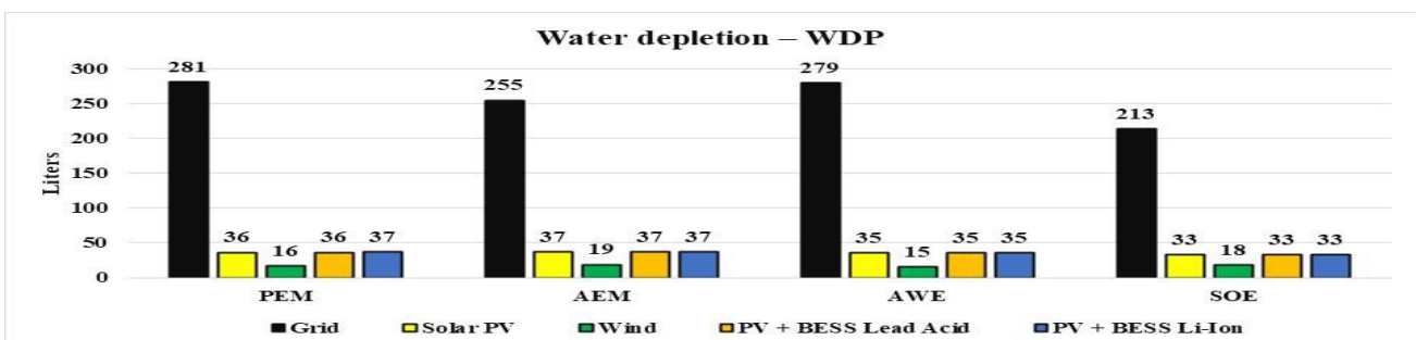
Figure 3 Water Depletion Potential (WDP)
